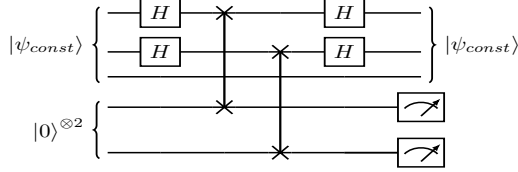
Fig. 20: SWAP based circuit for asserting constant set
